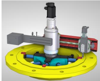
IN-SITU FLANGE FACER
